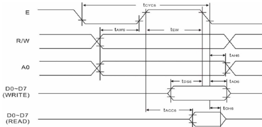
READ/WRITE TIMING FOR THE 68-PORT MPU
