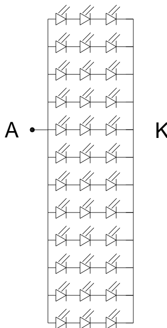
CIRCUIT DIAGRAM
